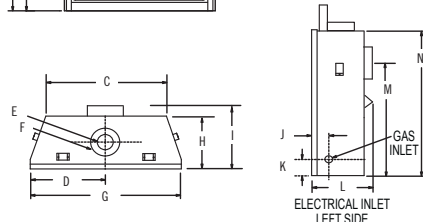
ELECTRICAL INLET LEFT SIDE
